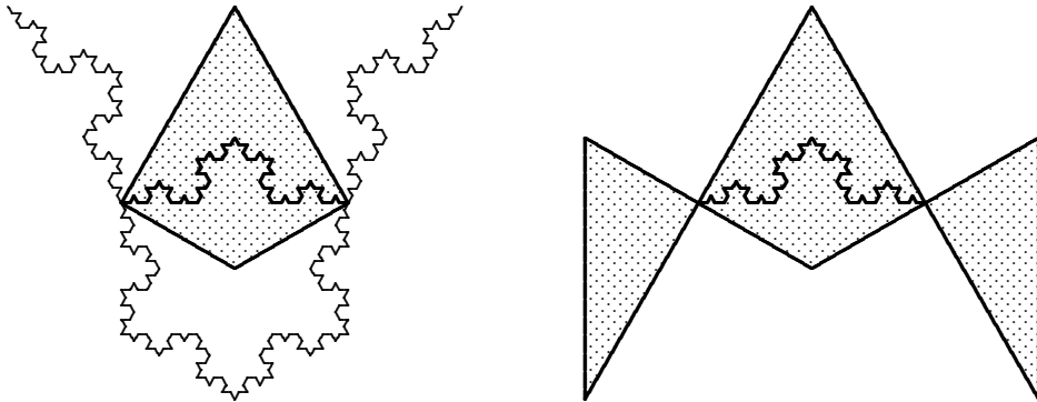
Figure 2. a) Neighbor sets and central open set for the Koch curve b) A feasible open set which contains the central one
