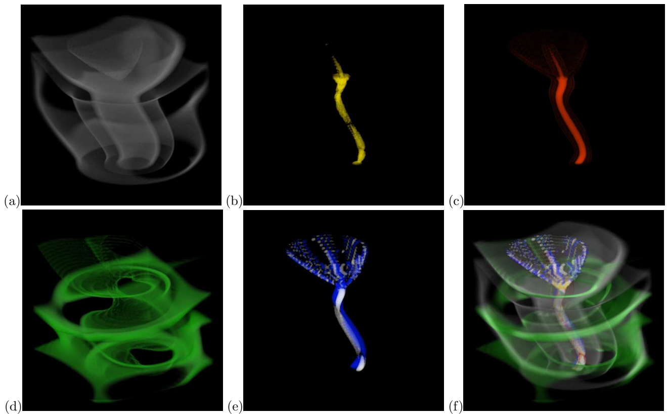
Figure 6. Feature extraction from tornado dataset selecting regions of (a) constant velocity, (b) high gradient tensor determinant, (c) high curl magnitude, (d) distinct helicity, (e) high negative (blue) and high positive (white) divergence, and (f) their combination using MDTF.
